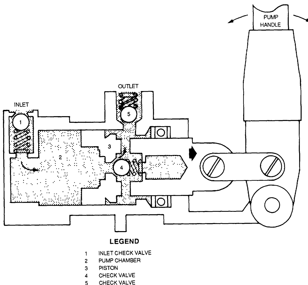
Figure 4-111. Double-Action Hand Pump
