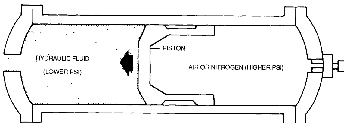
Figure 4-118. Cylindrical Accumulator
