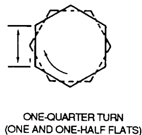
Figure 4-21. MS Turns and Torque Values
