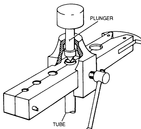
Figure 4-10. Flaring Tool
