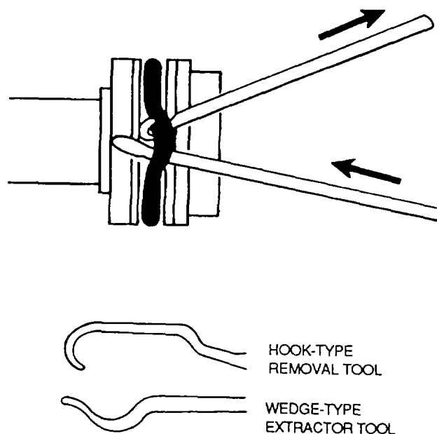
Figure 4-66. External O-Ring Removal (Wedge-Type Extractor)
