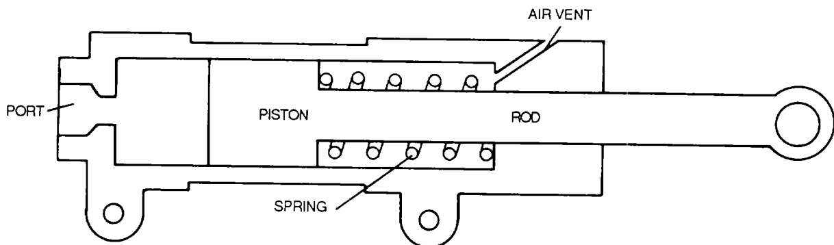
Figure 4-133. Single-Action Actuating Cylinder
