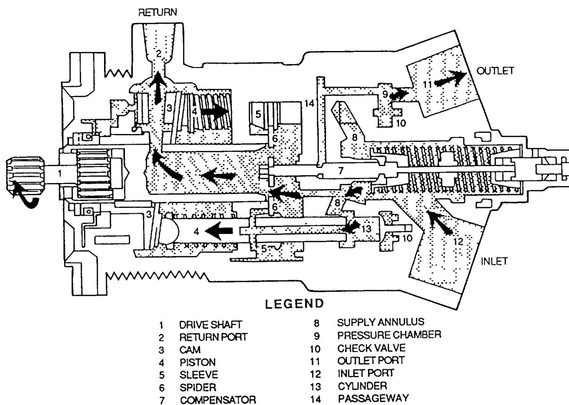
Figure 4-105. Stratopower Effective Stroke Pump (Full Flow)
