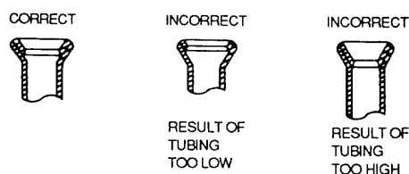
Figure 4-11. Tubing with Double Lap Flare
