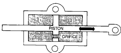
Figure 4-162. Piston Damper
