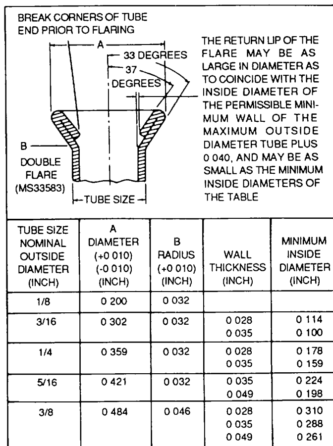
Figure 4-8. Dimensions for Double-Flared Tubing
