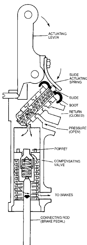
Figure 4-150. Power-Boost Master Cylinder (Brake Applied)
