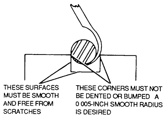
Figure 4-60. Removing O-Ring
