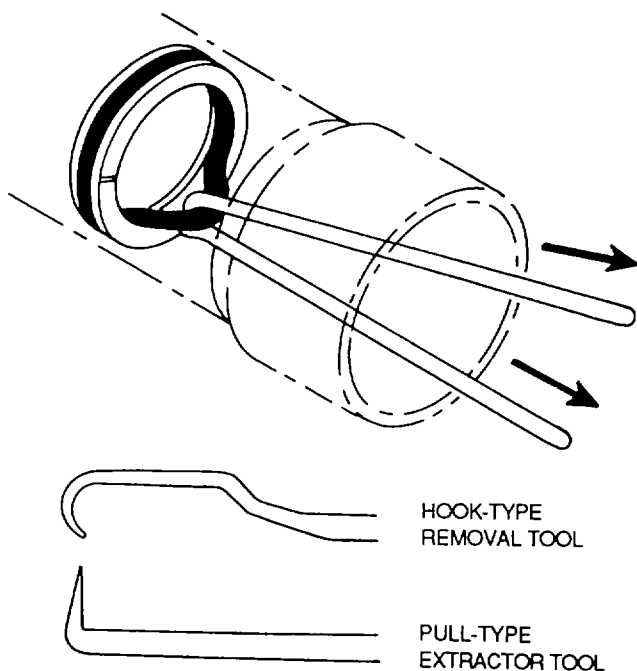
Figure 4-61. Internal O-Ring Removal (Pull-Type Extractor)
