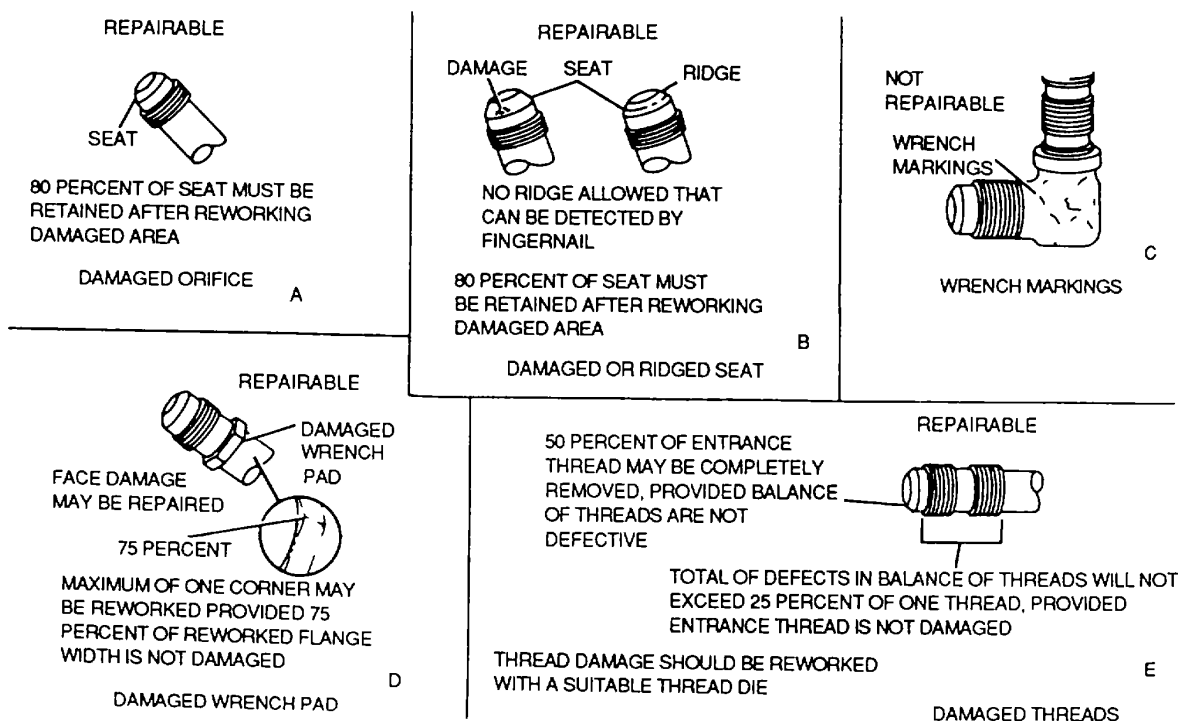
Figure 4-29. Damaged Fittings
