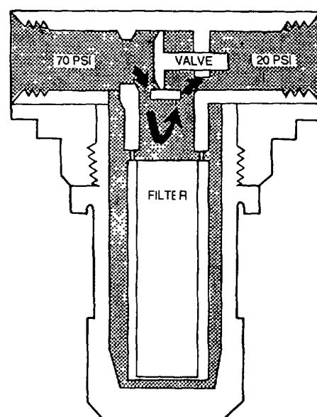
Figure 4-98. Fluid Filter (Clogged)
