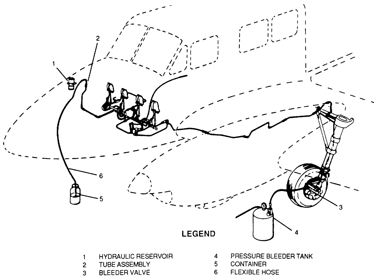
Figure 4-160. Bleeding Brake Hydraulic System
