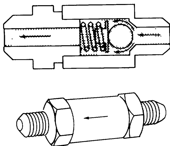
Figure 4-127. Simple Check Valve
