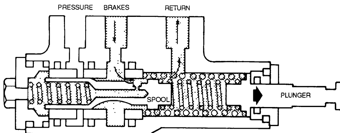
Figure 4-153. Power Brake Control Valve (Brakes Released)
