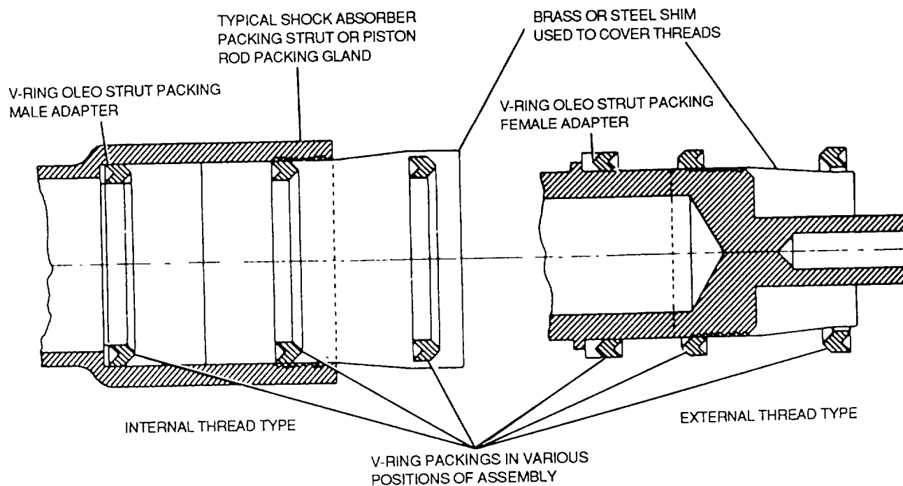
Figure 4-71. V-Ring Packings in Various Positions of Assembly
