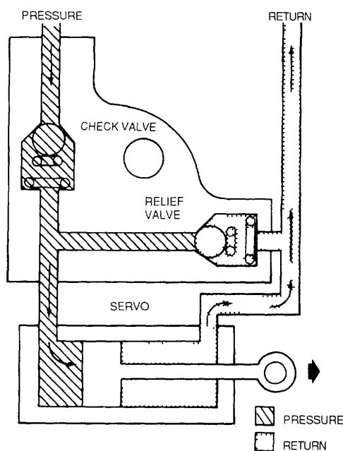
Figure 4-139. Irreversible Valve
