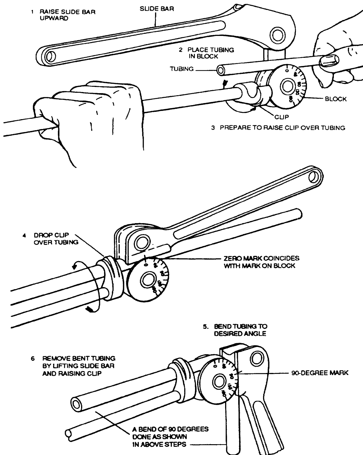
Figure 4-4. Bending Tube with Bending Machine
