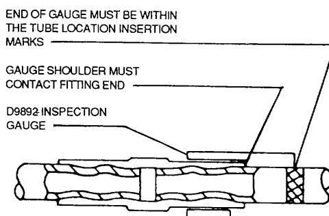
Figure 4-85. Checked Swaged Joint with D9892 Inspection Gauge
