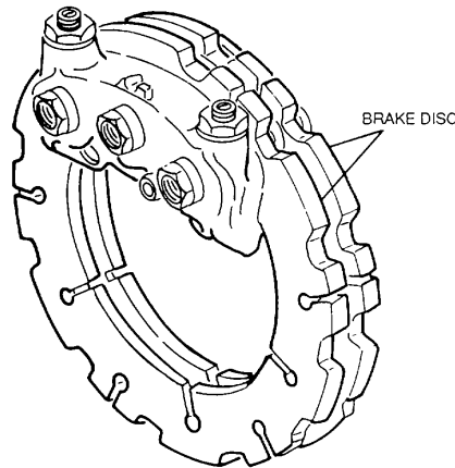
Figure 4-154. Disc Brake Assembly
