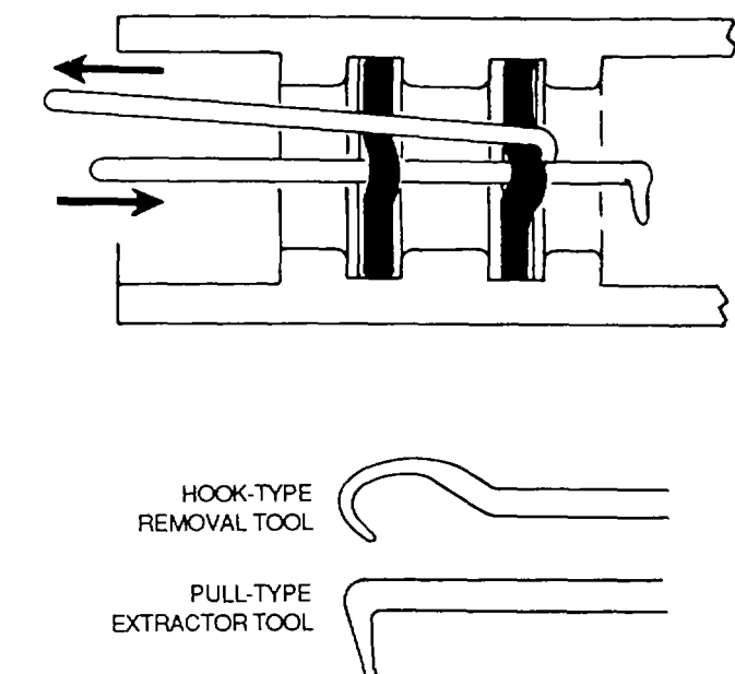
Figure 4-64. Dual Internal O-Ring Removal
