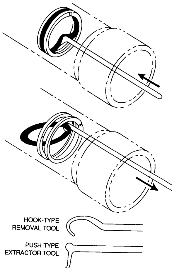
Figure 4-63. Internal O-Ring Removal (Push-Type Extractor)
