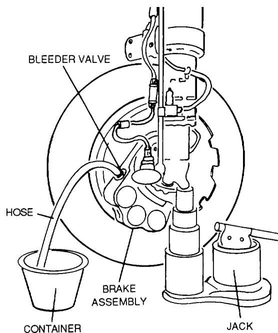
Figure 4-161. Gravity Method for Brake Bleeding
