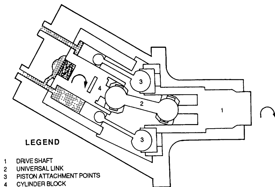
Figure 4-102. Constant Volume Pump (Piston Installation)
