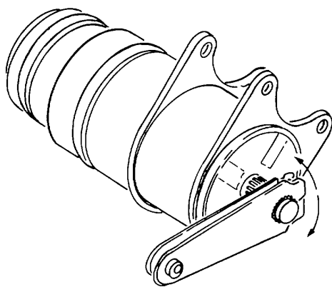
Figure 4-166. Vane Damper
