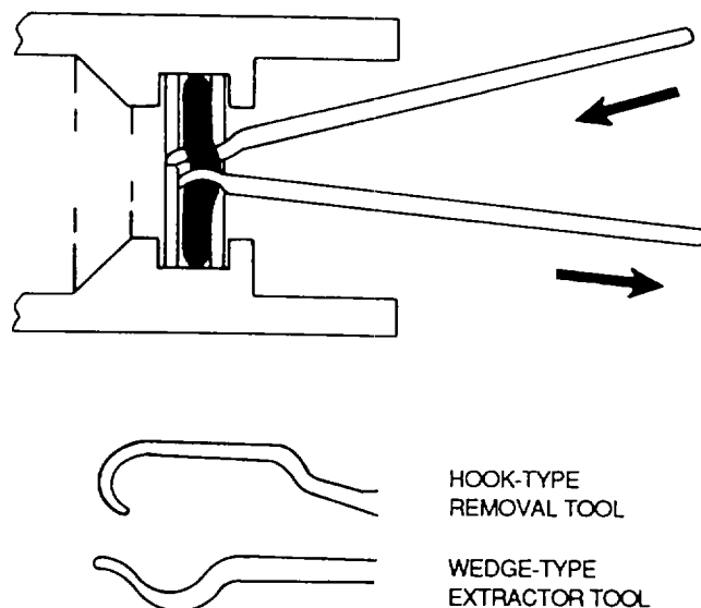
Figure 4-62. Internal O-Ring Removal (Wedge-Type Extractor)
