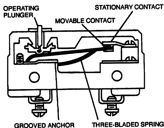
Figure 3-11. Microswitch
