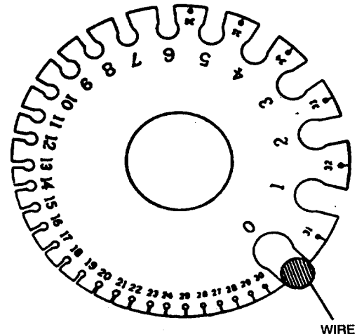
Figure 3-1. Wire Gauge
